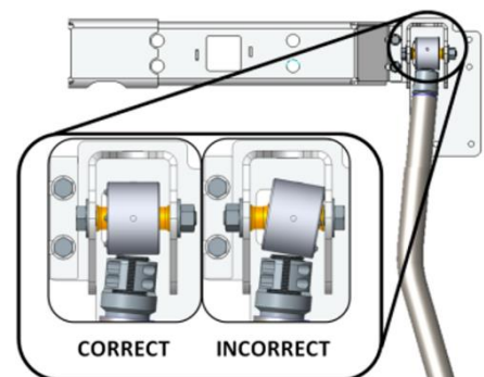
*Shown with suspension at ride height*
